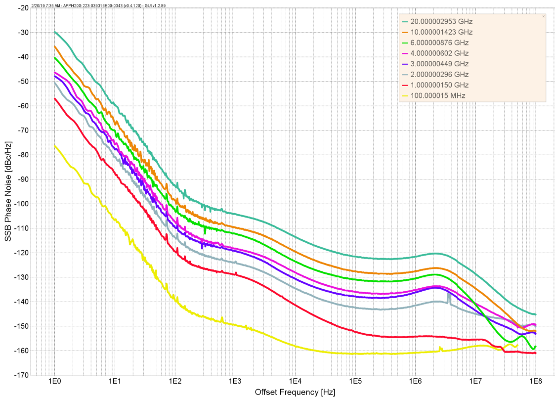
Figure 2: SSB Phase Noise Performance, CW without option LN, Pout=10 dBm
