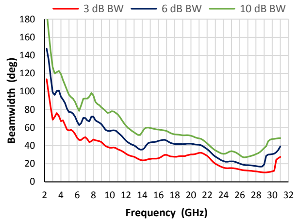
H plane
