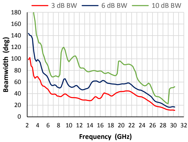
E plane
