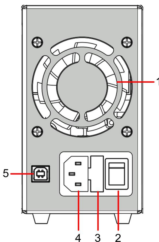
Figure 3-2 Rear Panel Overview (With USB model)
